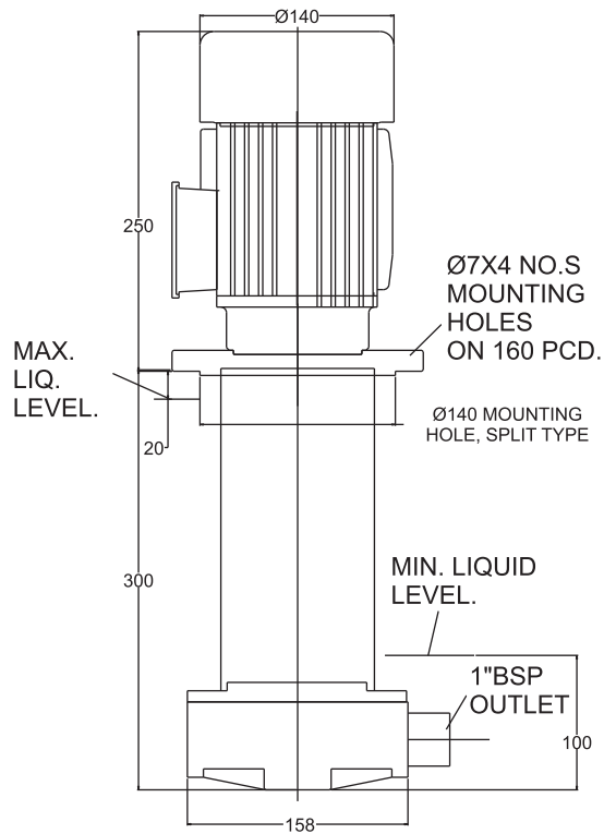
RPP160 in vertical immersion type. All wet ends in poly-propelene.
