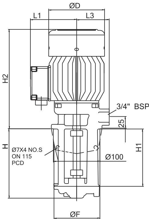
DIMENSIONAL DETAILS
