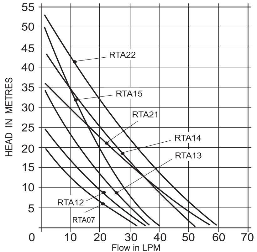
PERFORMANCE GRAPH
