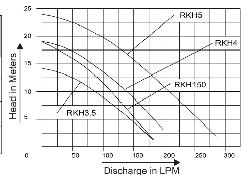
FOR RKH 150. Suction 1" BSP
